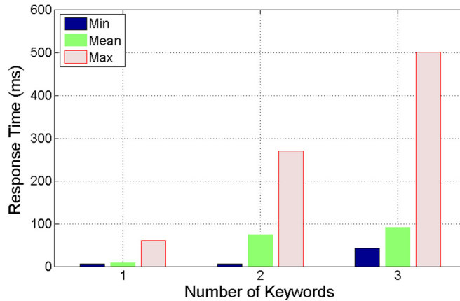
Fig. 9. The response time of the keyword-based localization process with respect to the increasing number of keywords.
