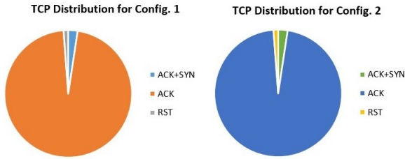
Fig. 2. TCP packet-types responsible for EED
