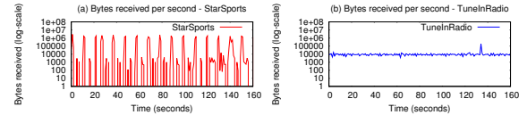
Fig. 3. Traffic Distribution for Streaming Apps Traffic
