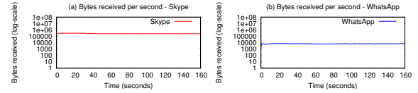
Fig. 1. Traffic Distribution for Interactive Apps Traffic
